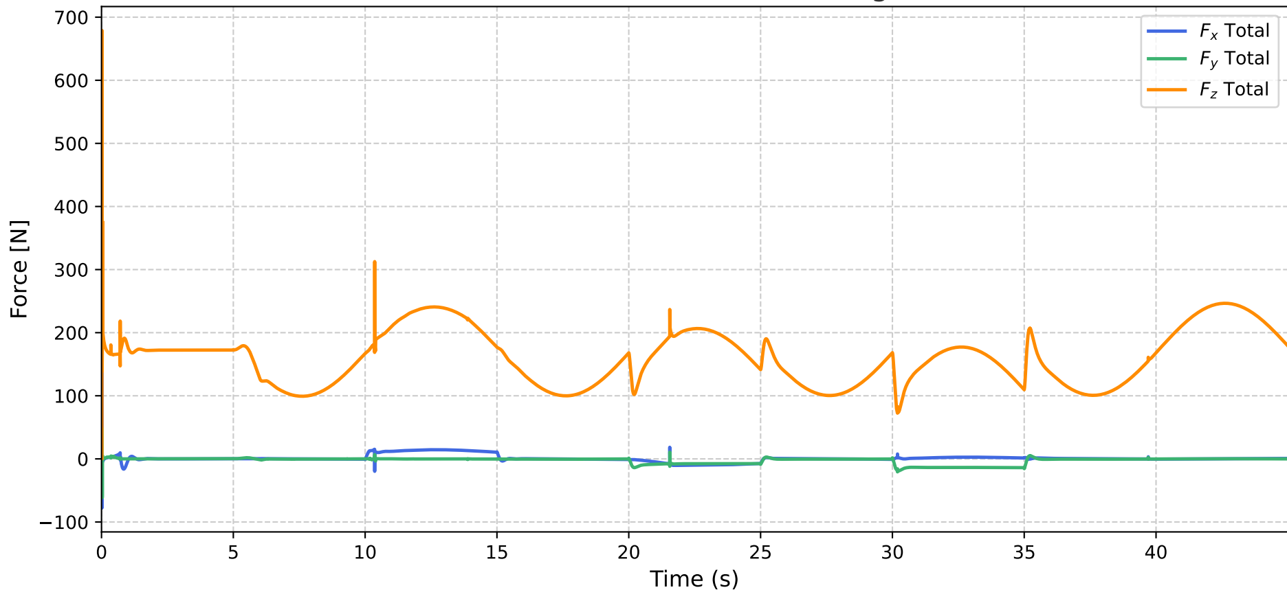
Total Ground Reaction Force – Right Foot
