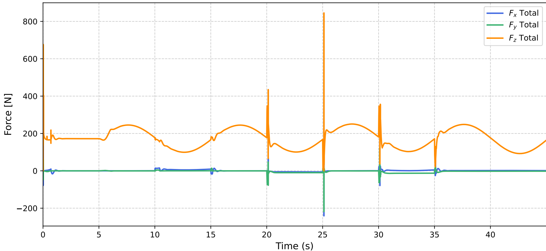
Total Ground Reaction Force - Left Foot
