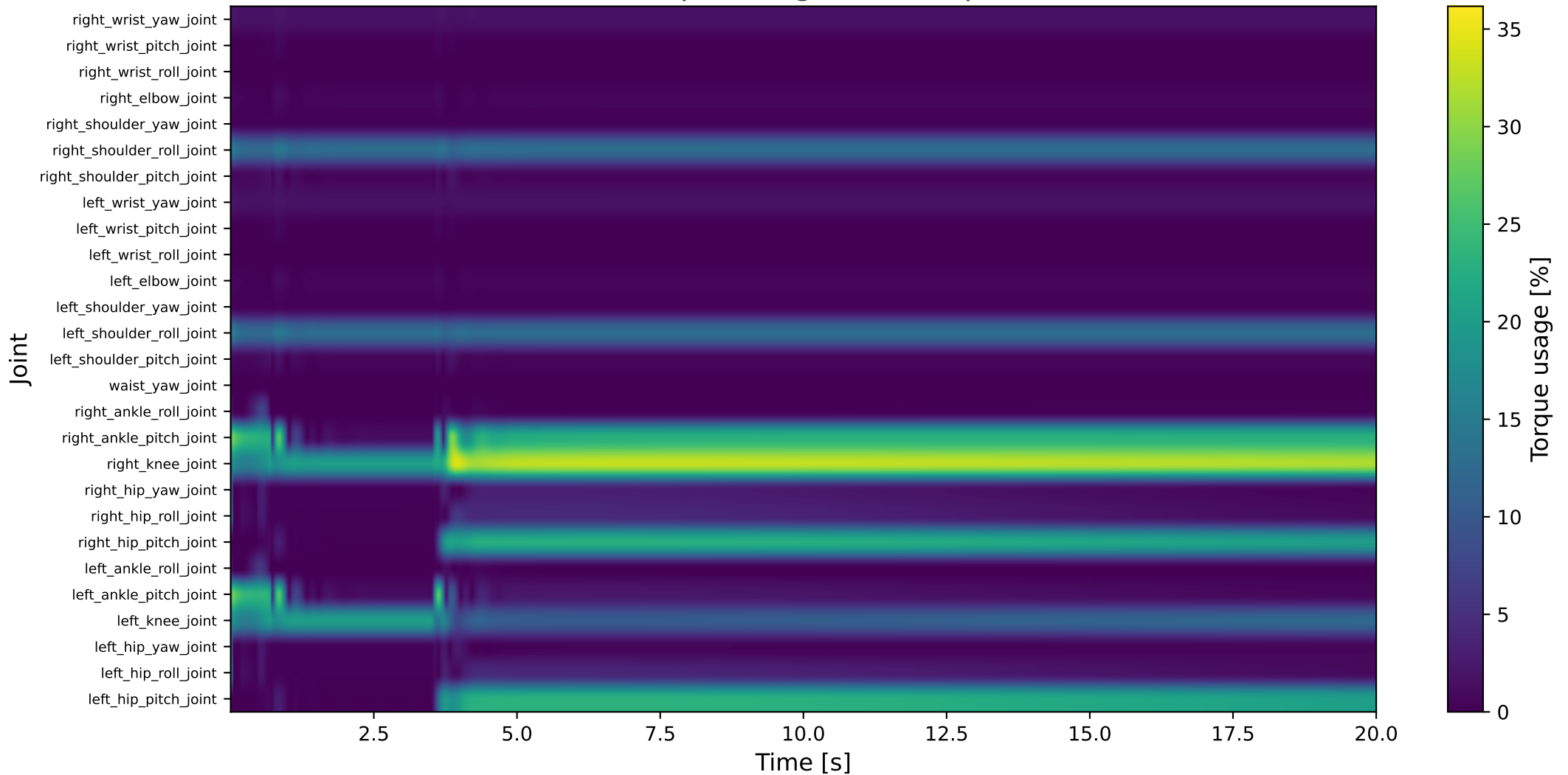
Torque usage heatmap
