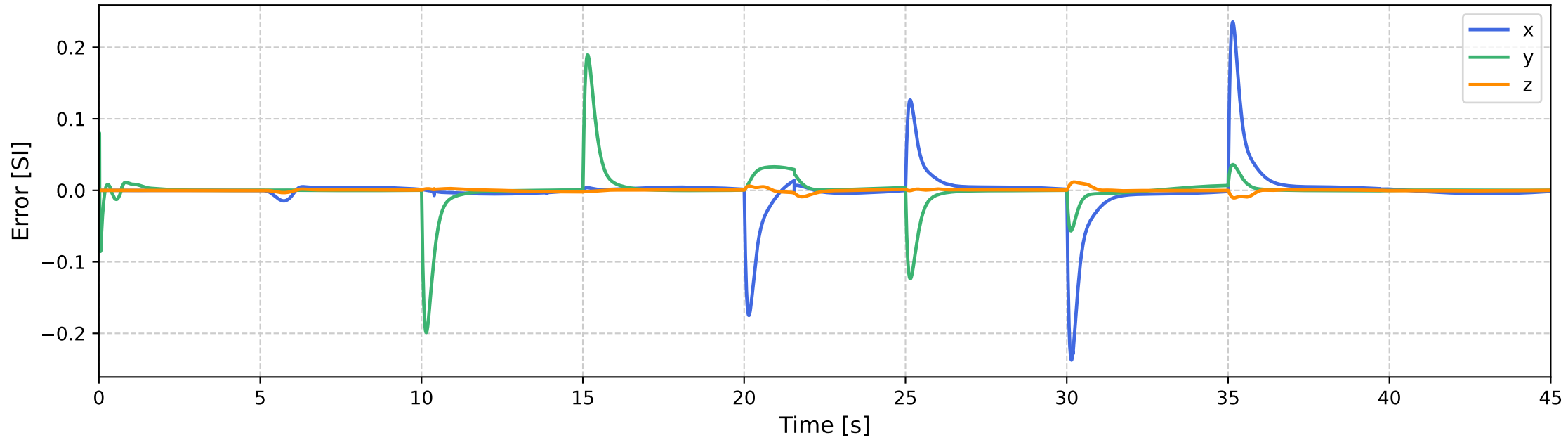
Velocity Error
