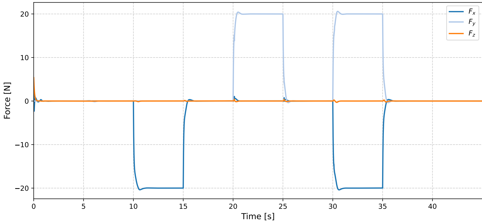
External Wrench - Forces
