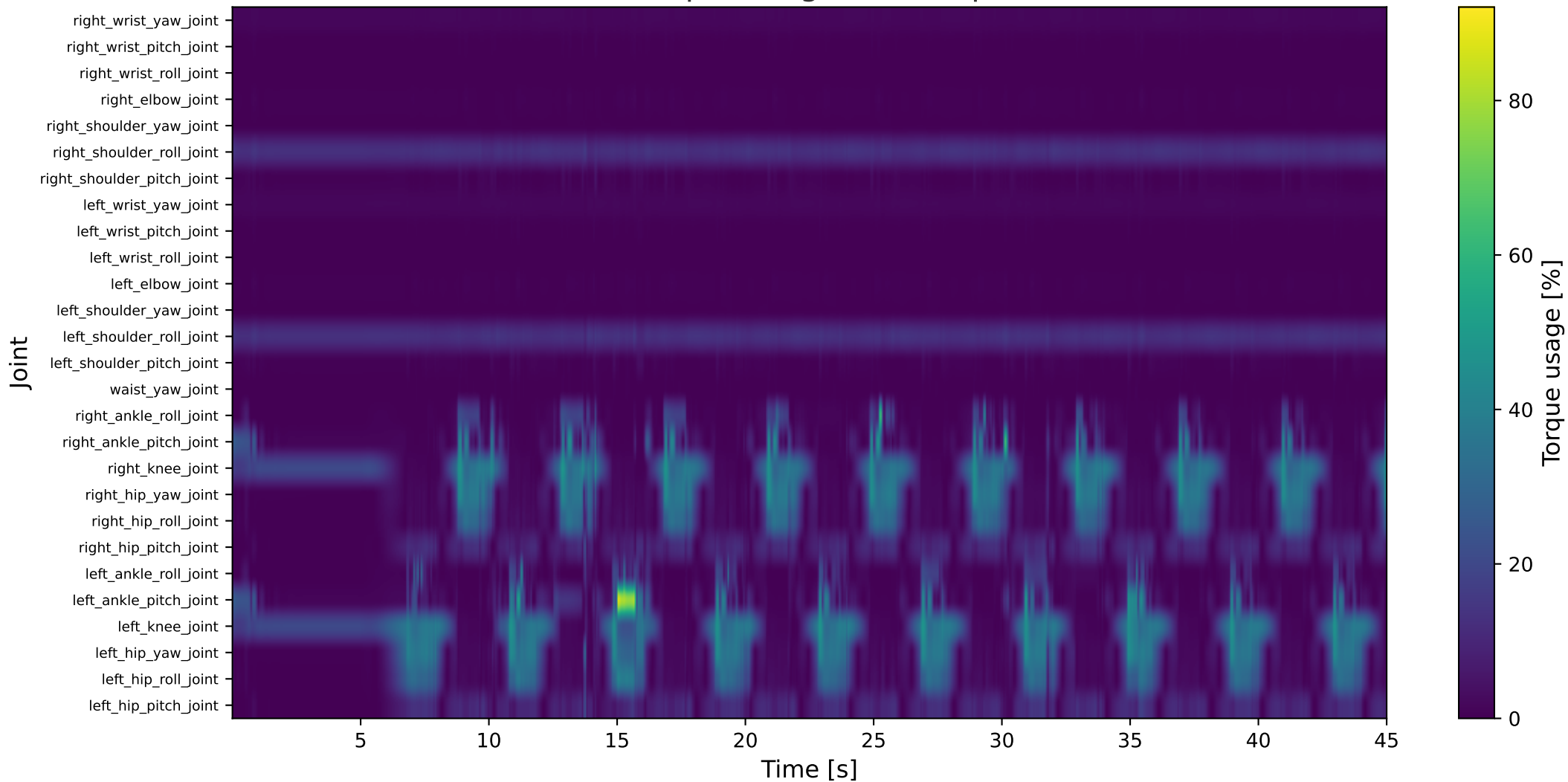
Torque usage heatmap
