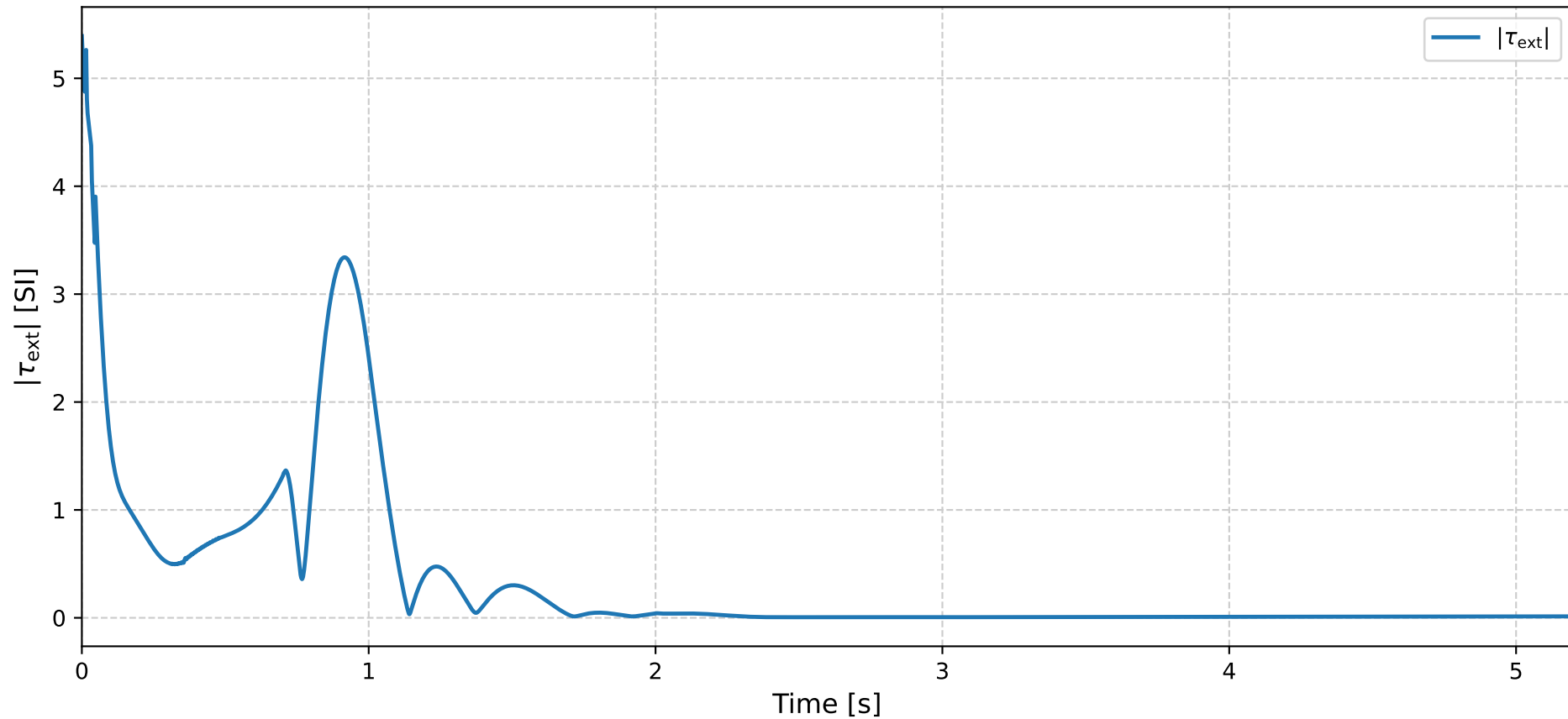
External Torque Norm ( \tau_{\text{ext}} )
