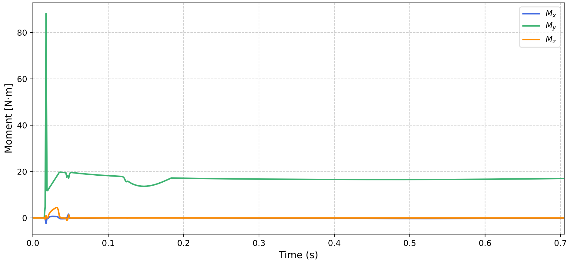
Total Ground Reaction Moment
