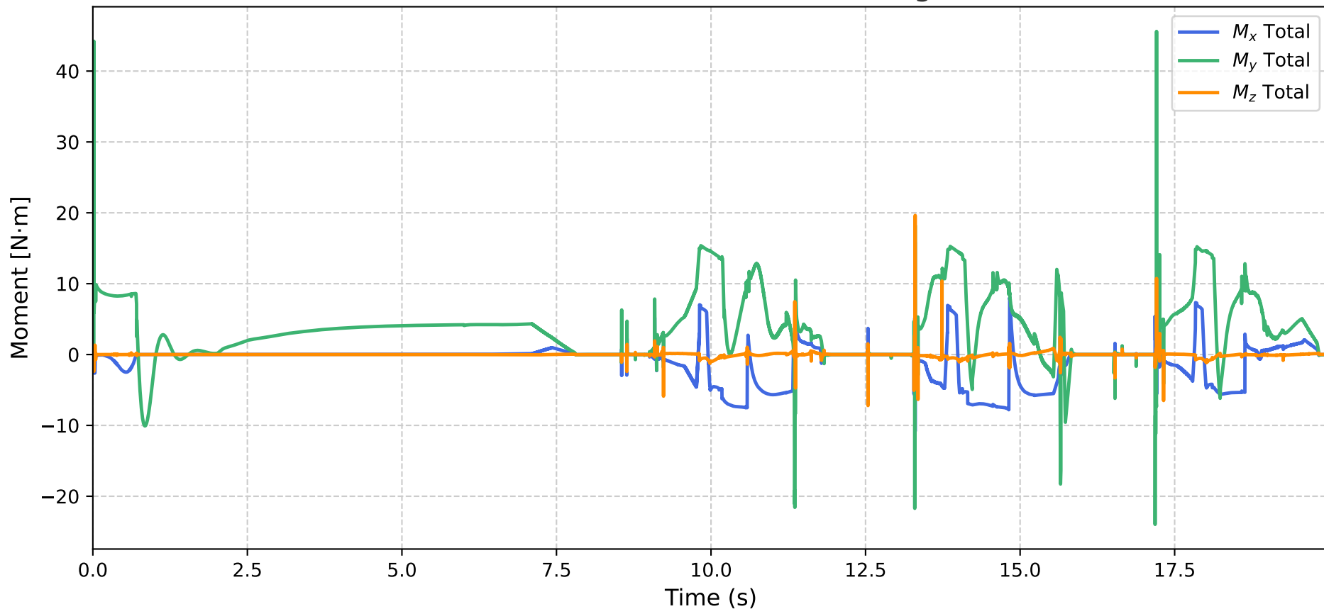
Total Ground Reaction Moment – Right Foot
