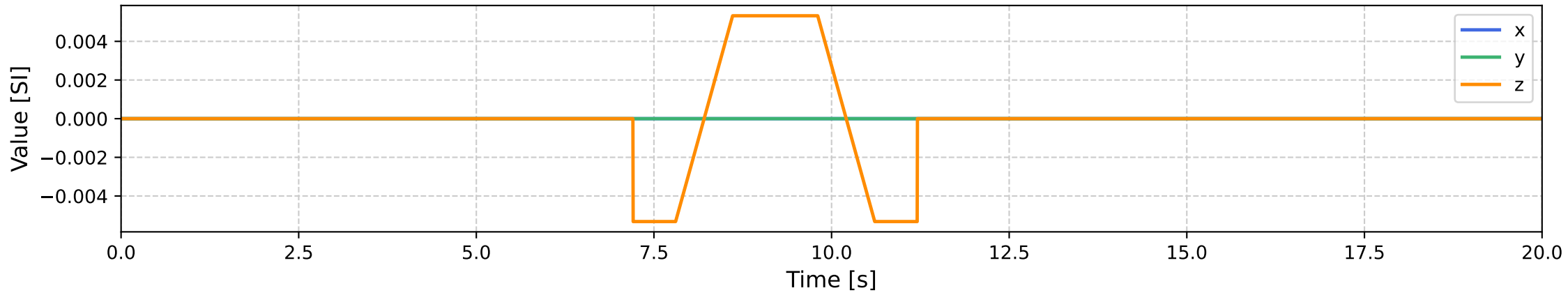
Desired Acceleration
