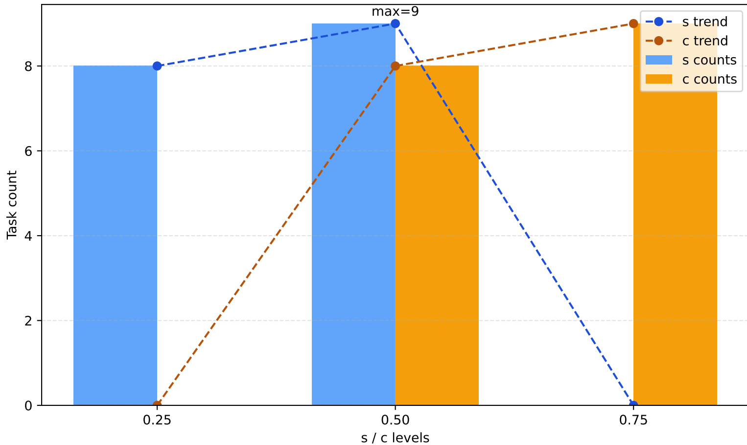
Authoritative s,c distribution
