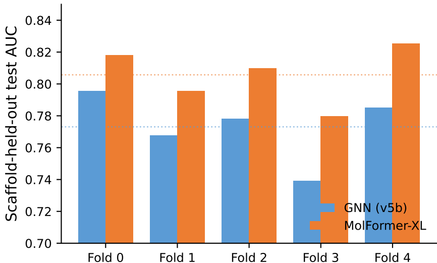
Per-fold test AUC across scaffold splits
