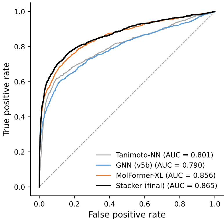
OOF ROC curves (n = 24,391)
