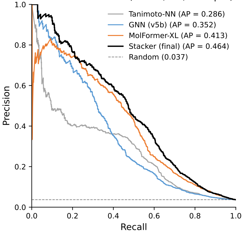
OOF Precision-Recall (n = 24,391, 3.7% pos)
