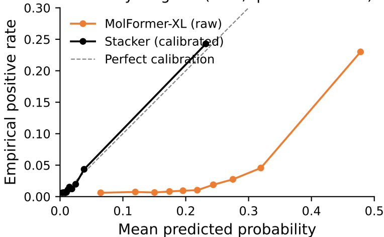
Reliability diagram (OOF, quantile-binned)
