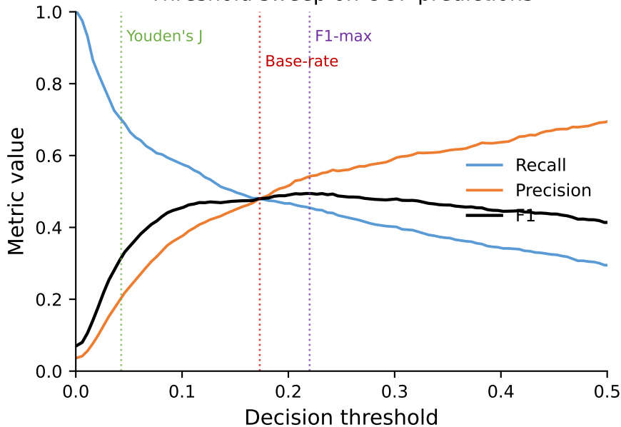
Threshold sweep on OOF predictions
