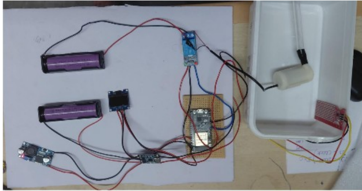
Fig. 5 - Assembled Prototype of the Solar-Powered Automated Dewatering System
