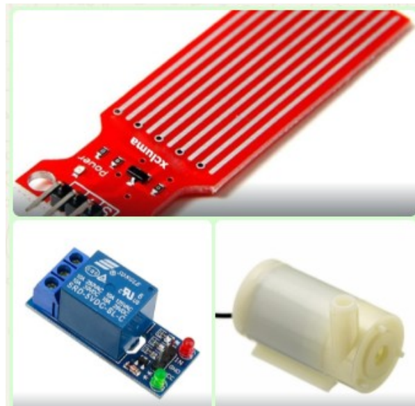
Fig. 1 - Core Components: Water-Level Sensor, Relay Module, and DC Motor Pump
