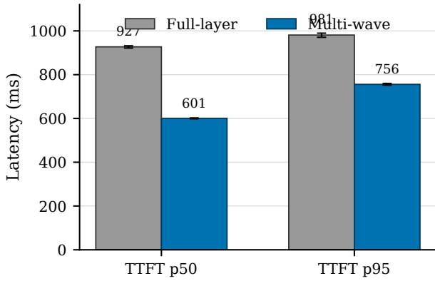
Figure 3. Capacity-bounded multi-wave staging reduces the repeat-median TTFT p50 by 35.21% and TTFT p95 by 22.96% relative to graph-compatible full-layer staging. Bars show the median of three independent service-start summaries; whiskers show their minimum and maximum. The comparison uses one Ascend 910B2, Qwen3-30B-A3B BF16, a 14-GiB offload target, 32 slots, and concurrency one.
