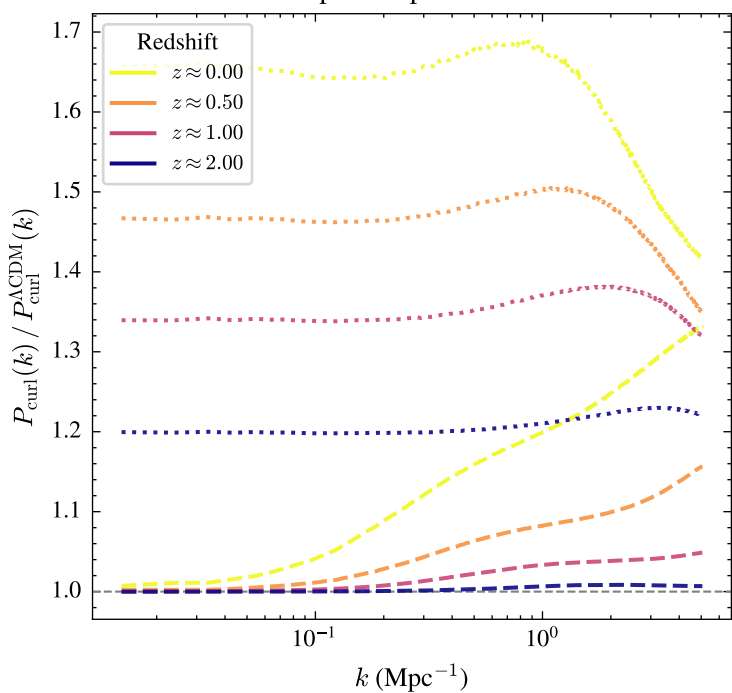
Curl power spectrum ratio
