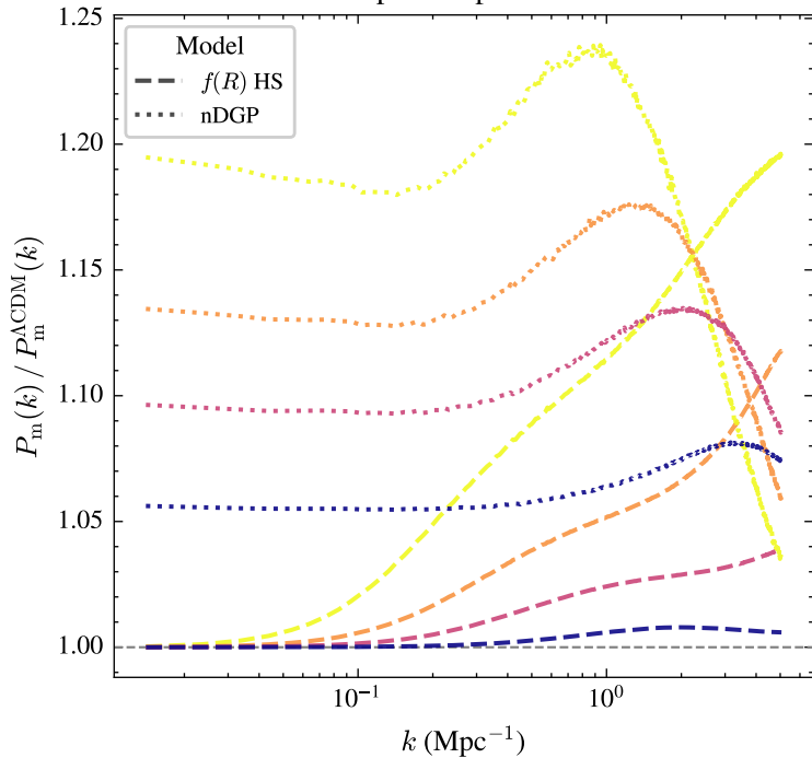
Matter power spectrum ratio
