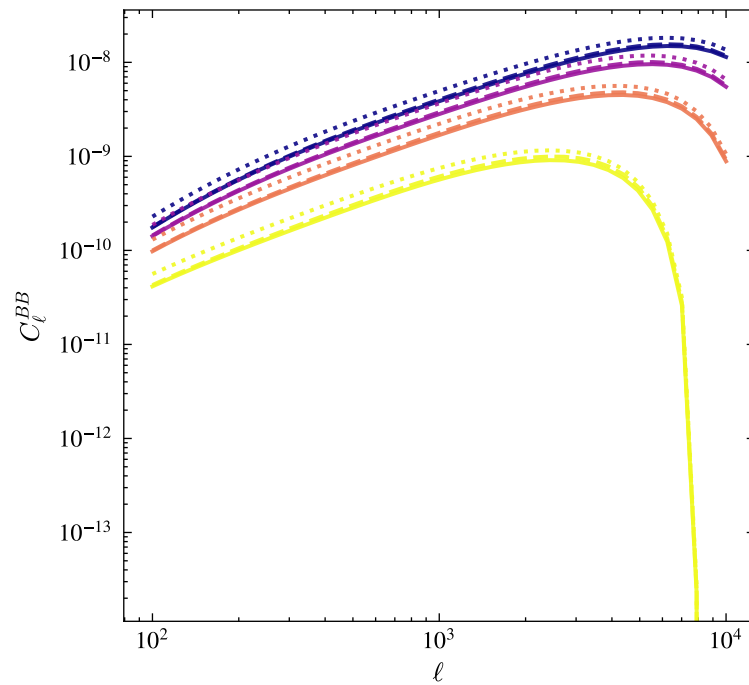
Gravitomagnetic BB
