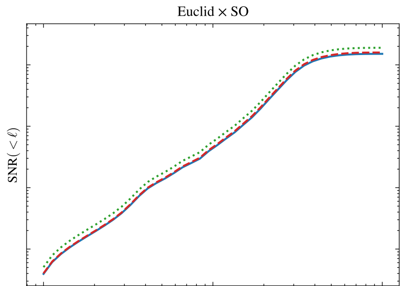
Cumulative SNR( < \ell_{\max} ) at z_s = 1.5
