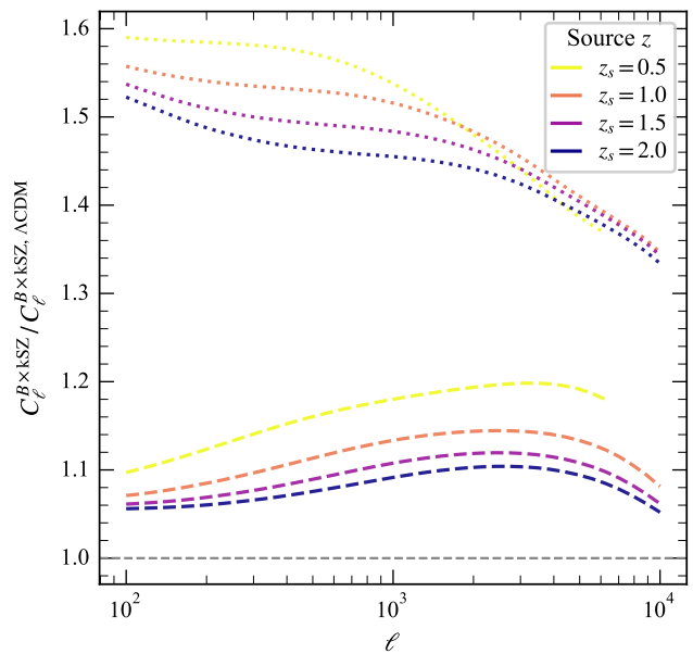
B \times kSZ ratio
