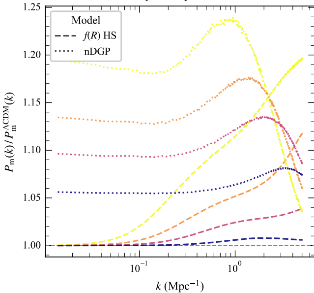
Matter power spectrum ratio
