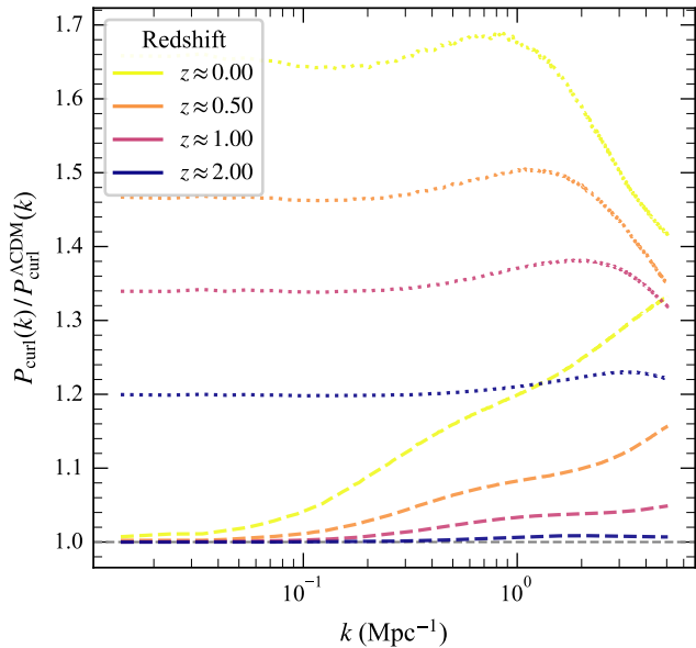
Curl power spectrum ratio
