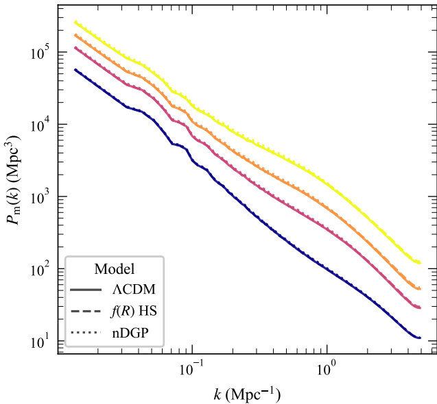
Matter power spectrum
