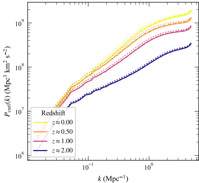
Curl (momentum) power spectrum
