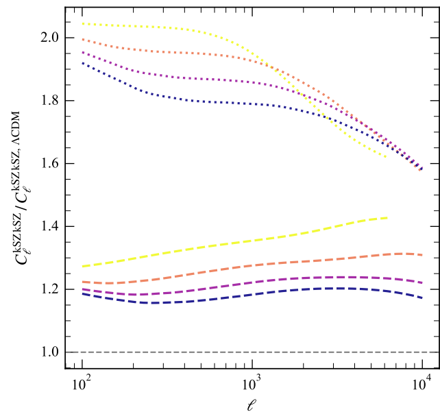
kSZ ratio
