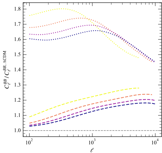
B \times \text{kSZ} ratio
