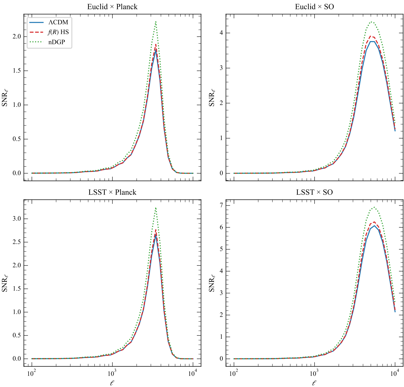
Per- \ell SNR at z_s = 1.5
