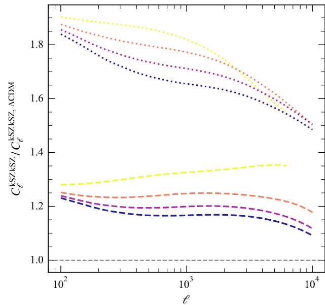
kSZ ratio
