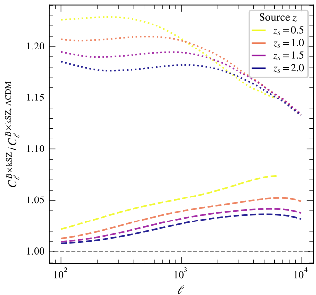
B \times \text{kSZ} ratio
