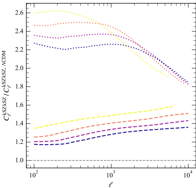
kSZ ratio
