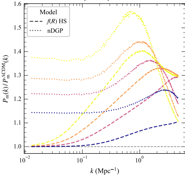
Matter power spectrum ratio
