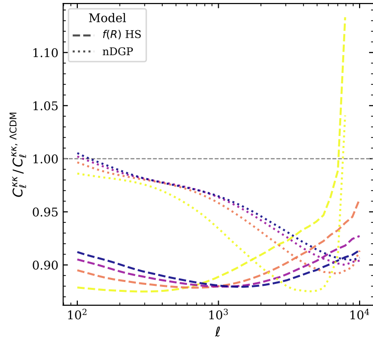
Lensing \kappa\kappa ratio
