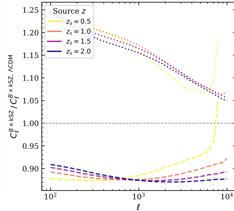
B \times \text{kSZ} ratio
