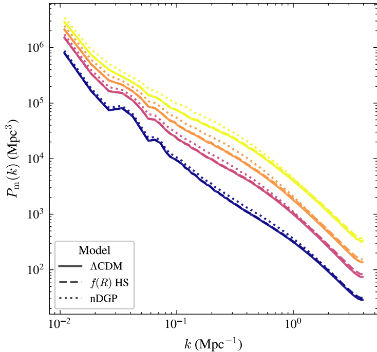
Matter power spectrum
