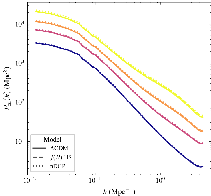
Matter power spectrum
