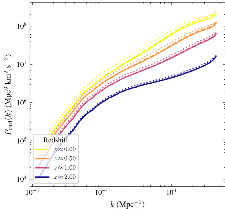
Curl (momentum) power spectrum
