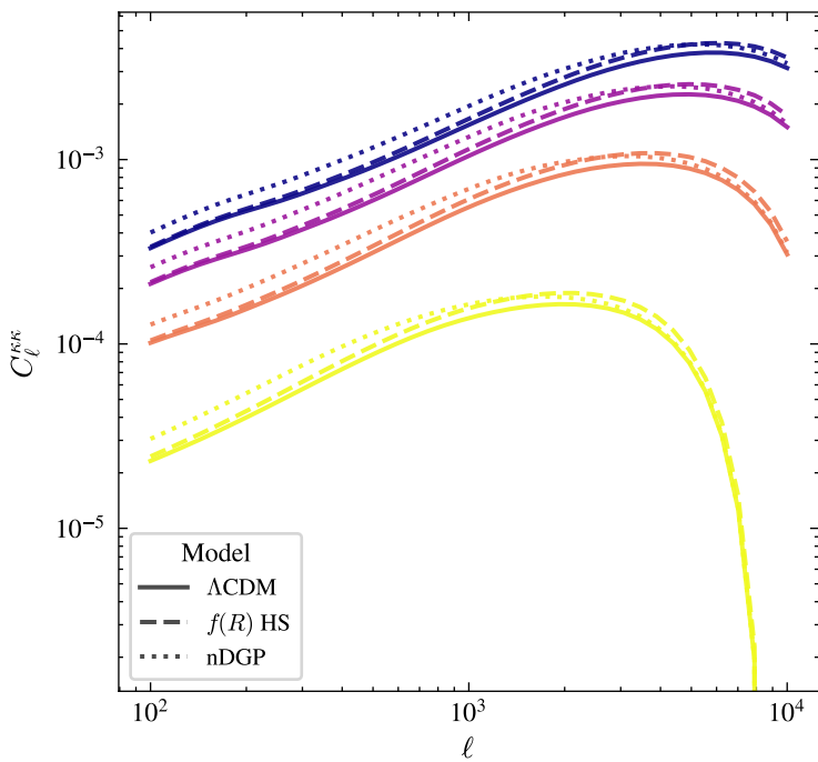
Lensing convergence \kappa\kappa
