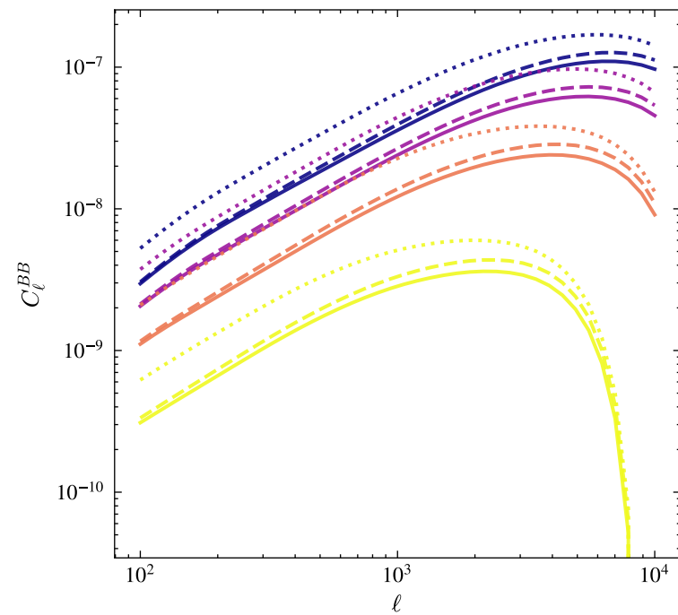
Gravitomagnetic BB
