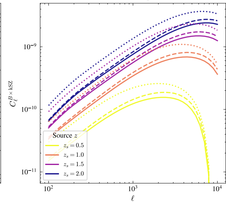
B \times kSZ cross-spectrum
