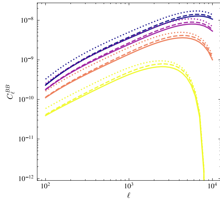
Gravitomagnetic BB
