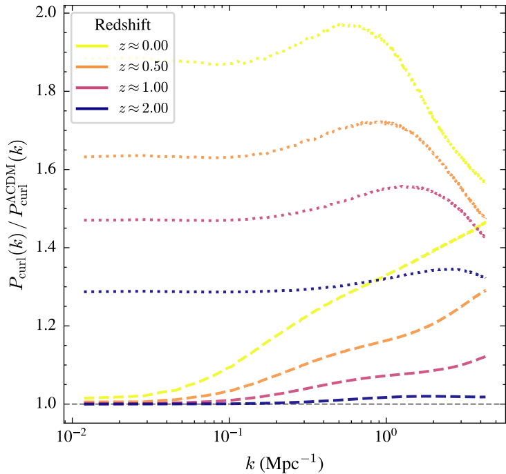
Curl power spectrum ratio
