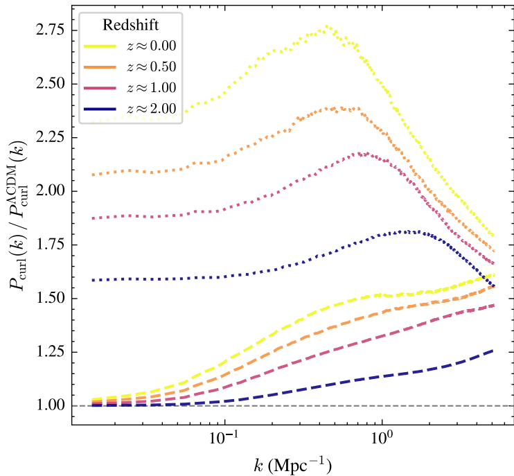
Curl power spectrum ratio
