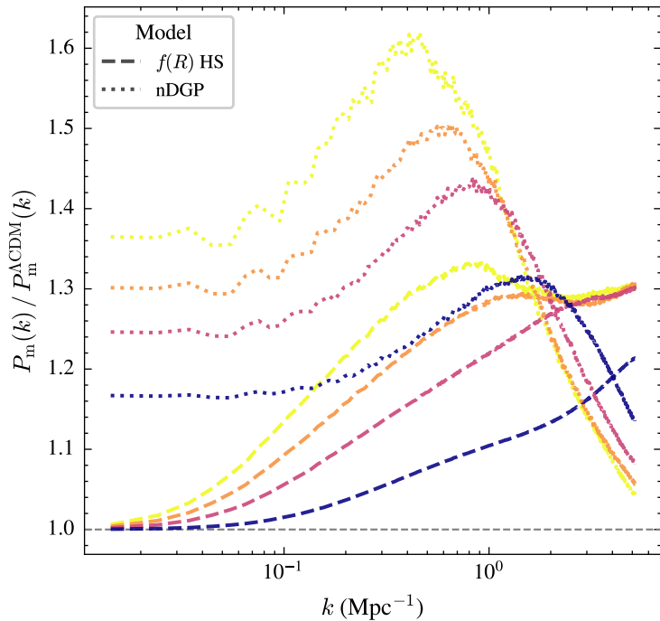
Matter power spectrum ratio
