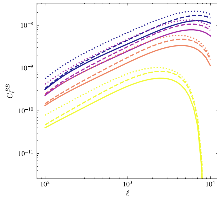
Gravitomagnetic BB
