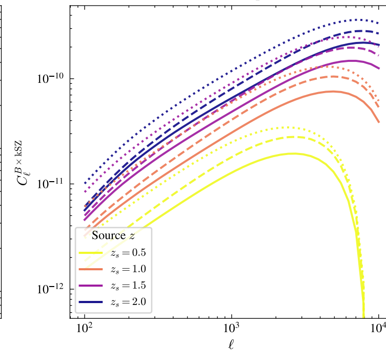
B \times kSZ cross-spectrum
