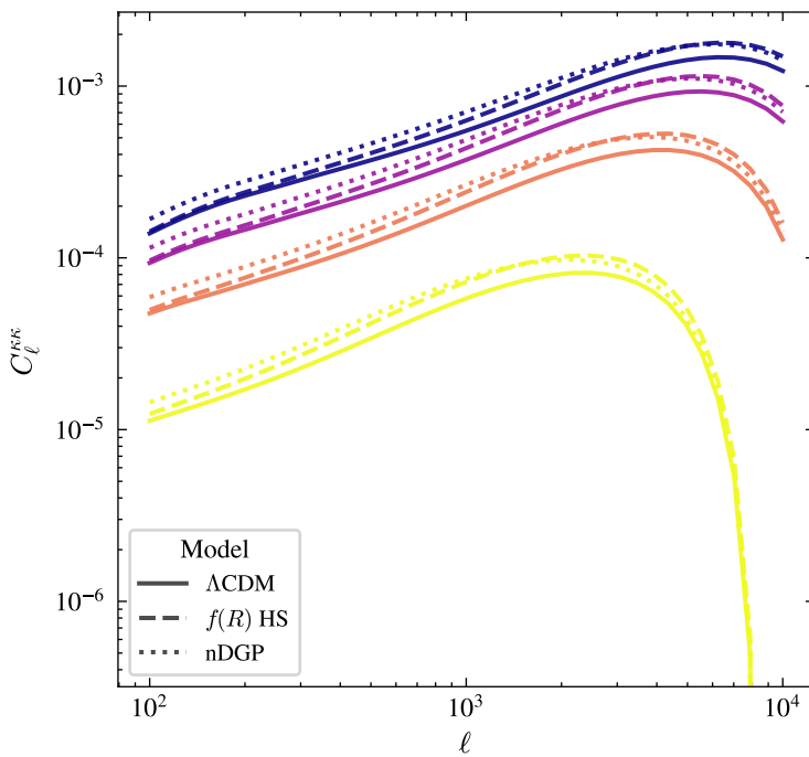
Lensing convergence \kappa\kappa
