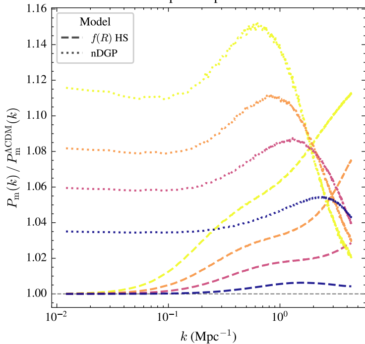
Matter power spectrum ratio
