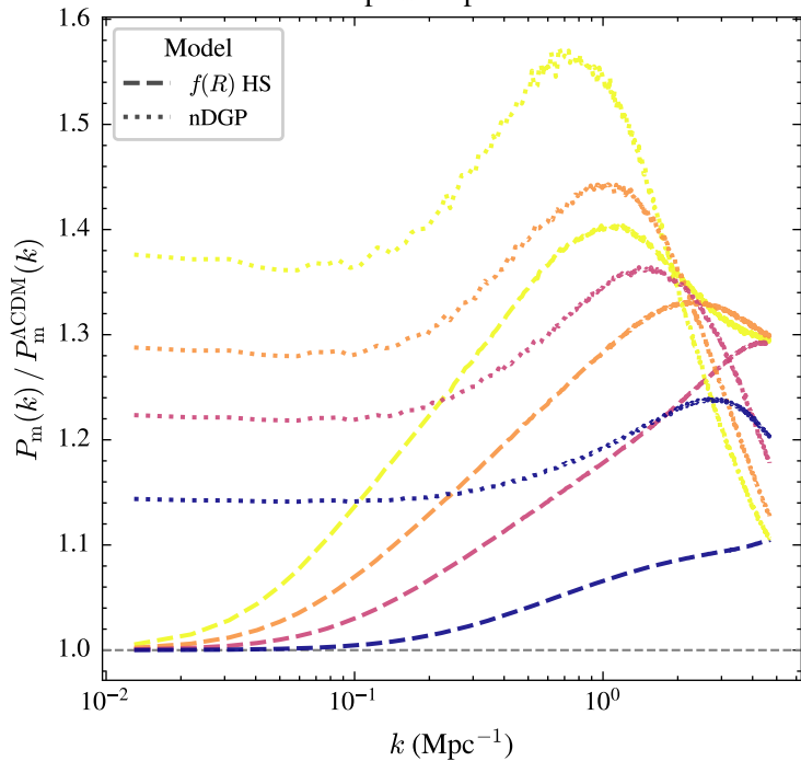
Matter power spectrum ratio
