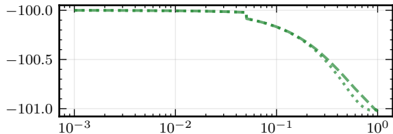
Scale factor a
