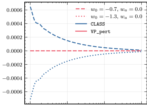
Velocity Perturbation V_{\text{DE}}(z)
