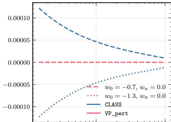
Velocity Perturbation V_{\text{DE}}(a)
