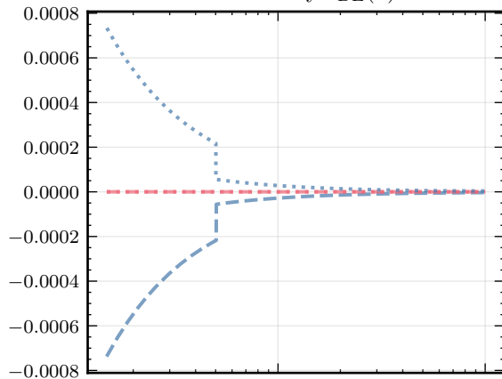
Overdensity \delta_{\text{DE}}(a)
