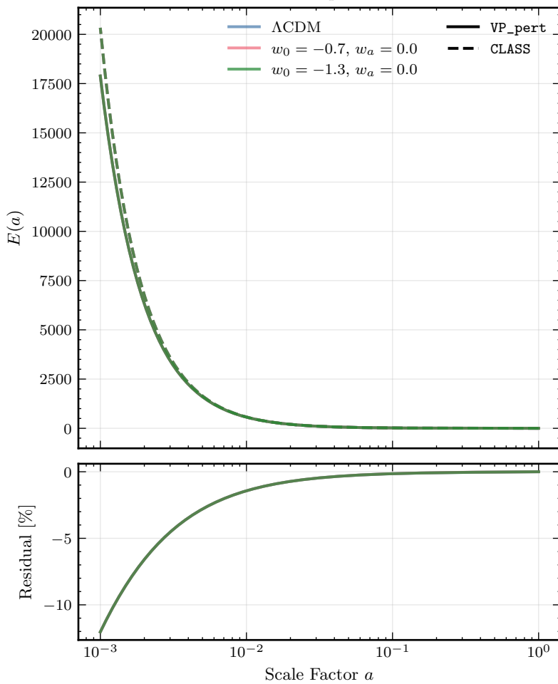
No radiation compared to CLASS
