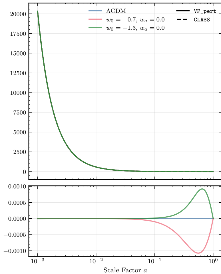
Radiation compared to CLASS
