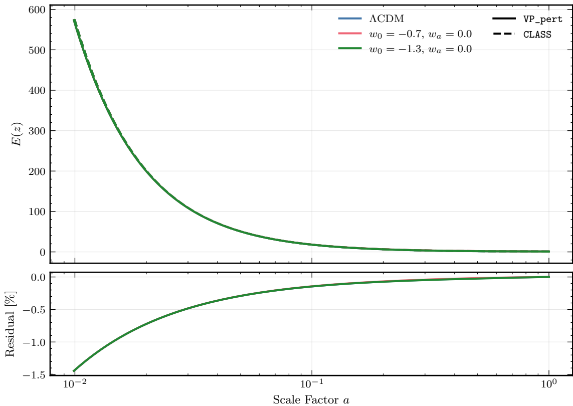
Dimensionless Hubble Rate
