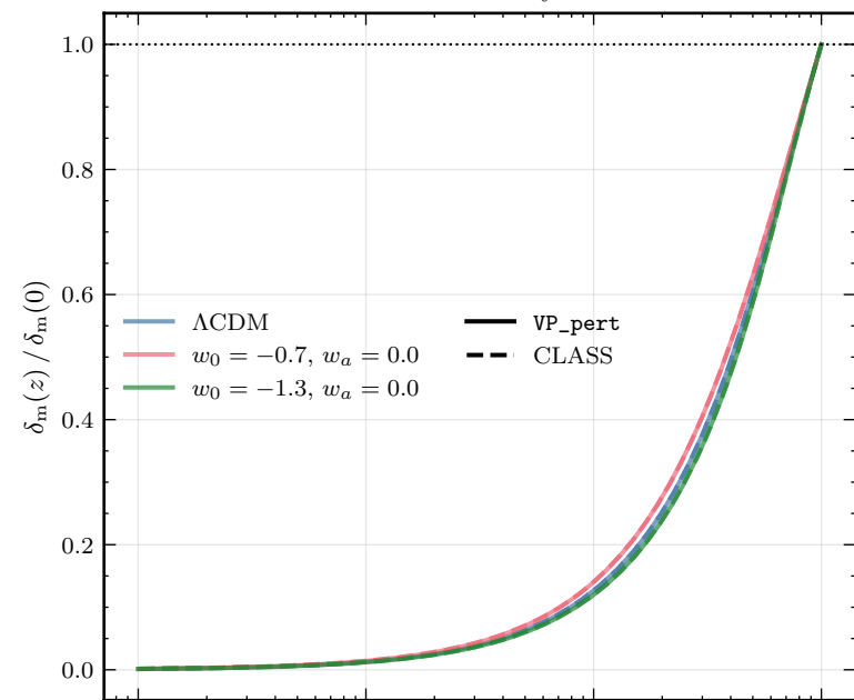
Overdensity
