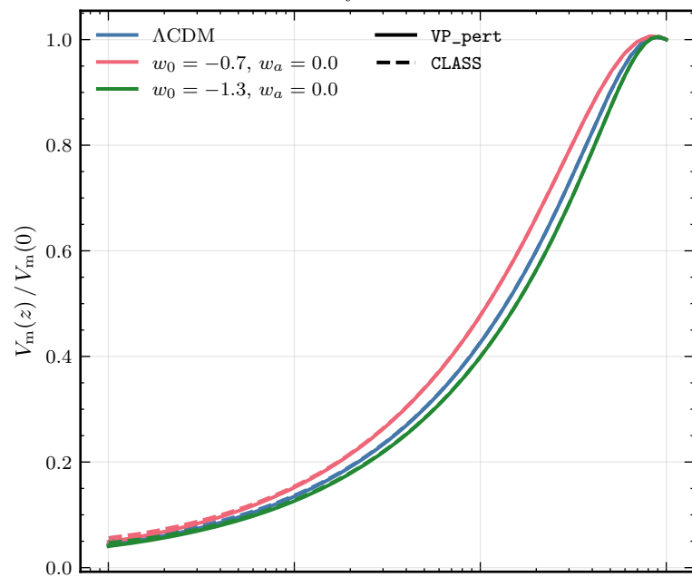
Velocity Perturbation
