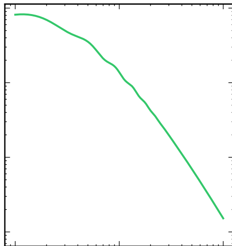
f(R) Hu-Sawicki
