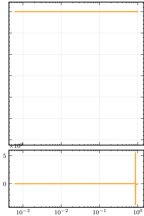
Cubic Galileon
