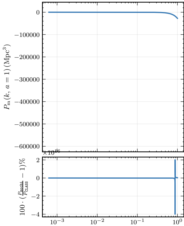
\Lambda CDM
