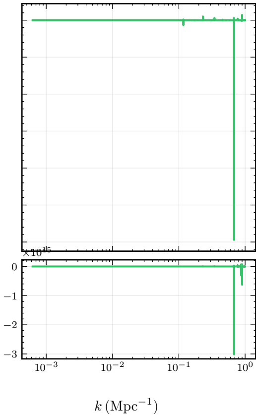
f(R) Hu-Sawicki
