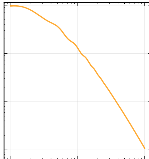
Cubic Galileon
