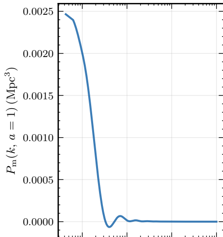
CLASS \Lambda CDM
