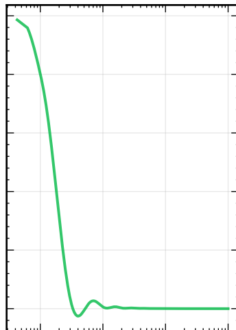
\Lambda CDM
